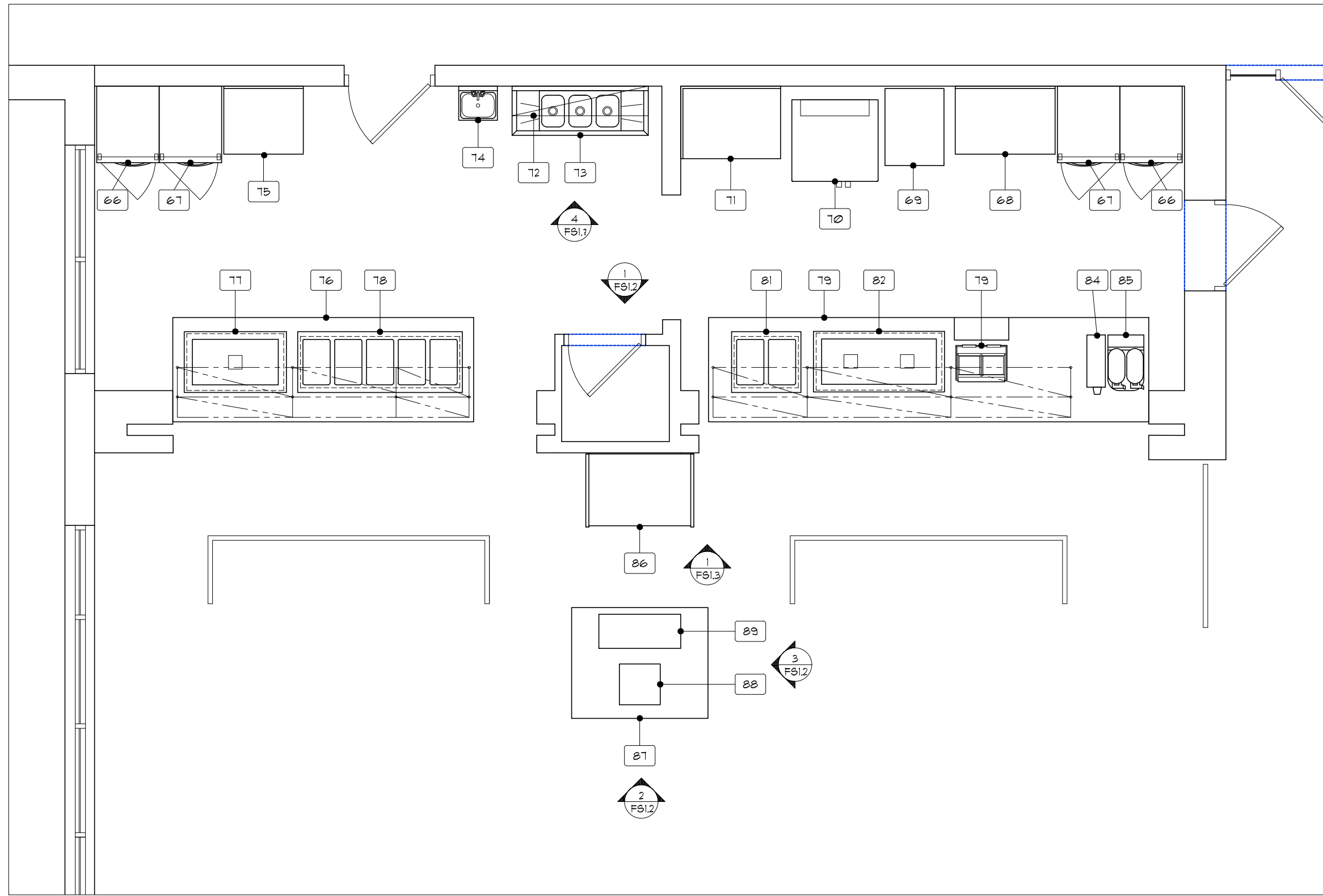
2 FOODSERVICE EQUIPMENT ARRANGEMENT PLAN
